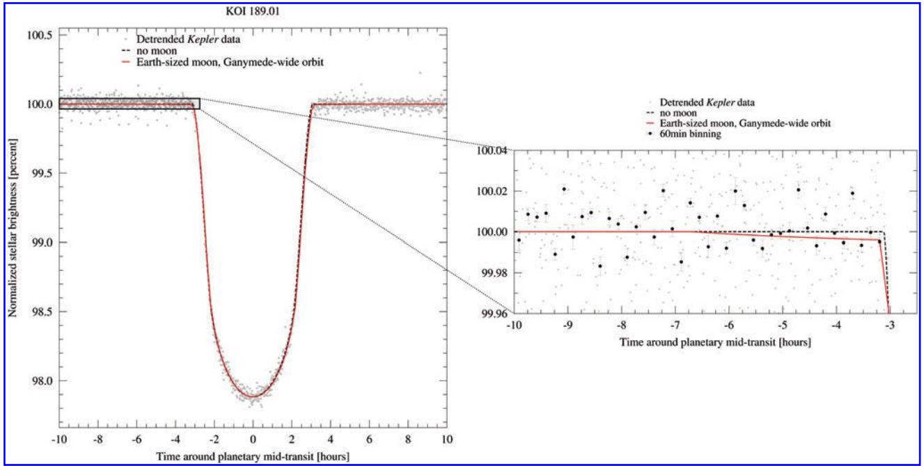
FIG. 13. Transit of the almost Jupiter-sized planet candidate KOI189.01 around a star of about 0.7 solar radii. Gray dots indicate the original phase-folded Kepler light curve, the black dashed line indicates a model for the transit assuming a planet only, and the red line assumes an Earth-sized moon in an orbit that is 15 planetary radii wide. Black dots in the right panel indicate data that is binned to 60 min. The photometric orbital sampling effect appears in the right panel as a deviation between the red solid and the black dashed line about 6.5 h before the planetary midtransit. (Color graphics available online at www.liebertonline.com/ast )
