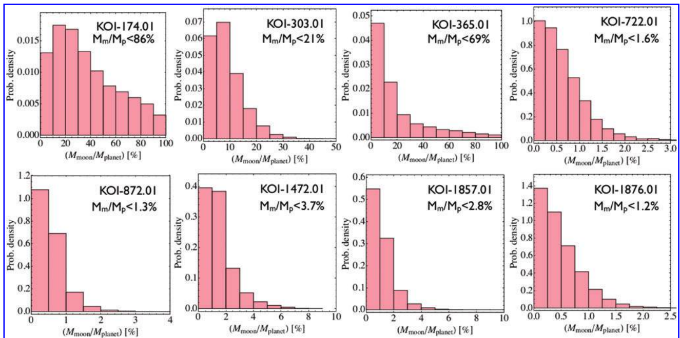
FIG. 17. Moon-to-planet mass ratio constraints derived so far by the HEK project (Nesvorný et al. , 2012; Kipping et al. , 2013a). Kepler-22b has also been studied and yields M_s < 0.5 M_\oplus but is not shown here, as the paper is still under review at the time of writing. (Color graphics available online at www.liebertonline.com/ast )
