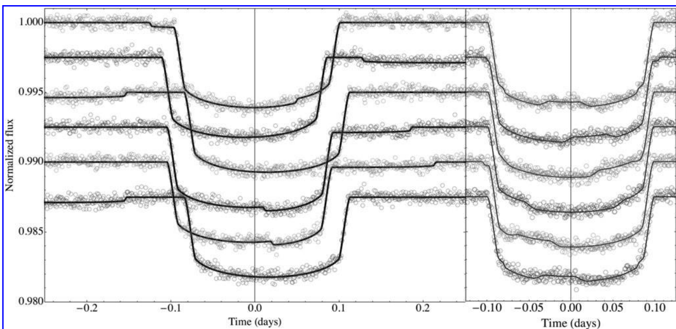
FIG. 12. (Left) Six simulated transits using LUNA (Kipping, 2011b) of a HZ Neptune around an M2 star with an Earth-like moon on a wide orbit (90% of the Hill radius). The moon can be seen to exhibit “auxiliary transits” and induce TTV. (Right) Same as left, except the moon is now on a close-in orbit (5% of the Hill radius), causing “mutual events.” Both plots show typical Kepler noise properties for a 12 th -magnitude star observed in short cadence.
