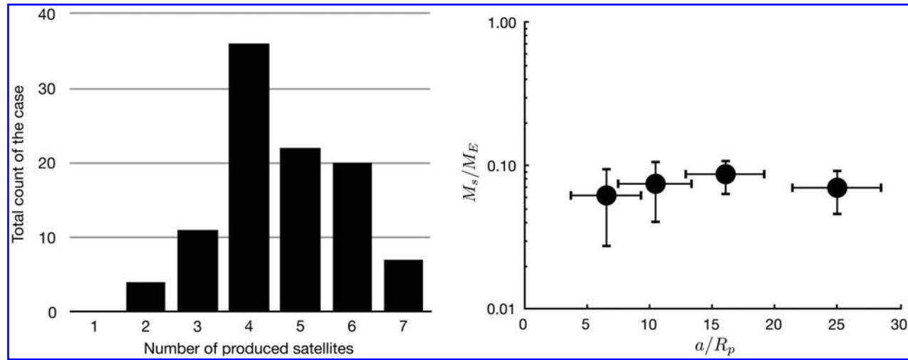
FIG. 2. Results after 100 simulations of moon formation around a 10 M_{\text{Jup}} planet. Left panel: Multiplicity distribution of the produced satellite systems for satellite masses M_s > 10^{-2} M_{\oplus} . Right panel: Averaged M_s and semimajor axis ( a ) are shown as filled circles; their standard deviations are indicated by error bars for the 36 four-satellite systems.
